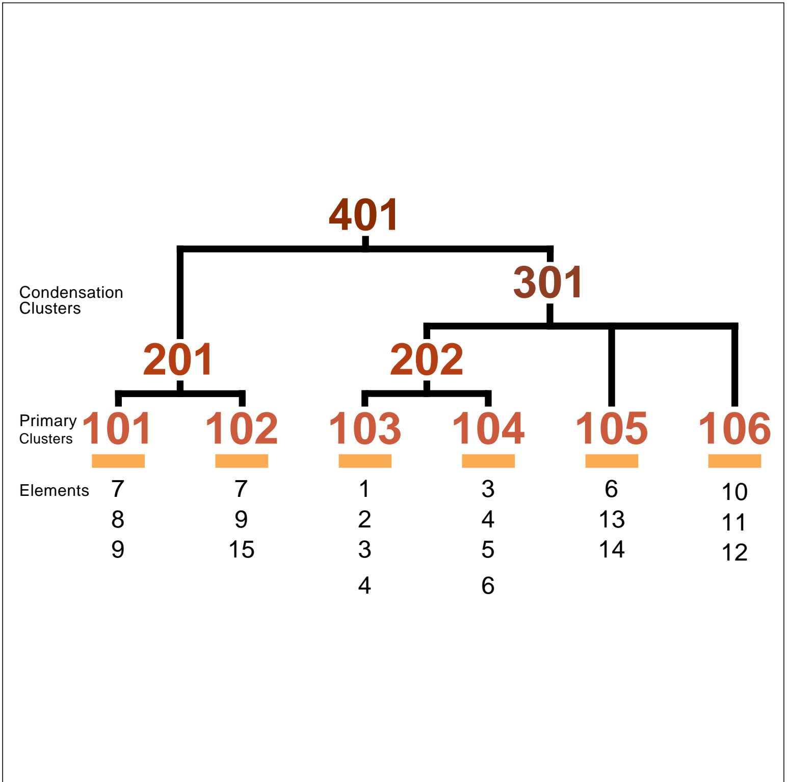
Figure 5 Clusters grouped into a hierarchy.
