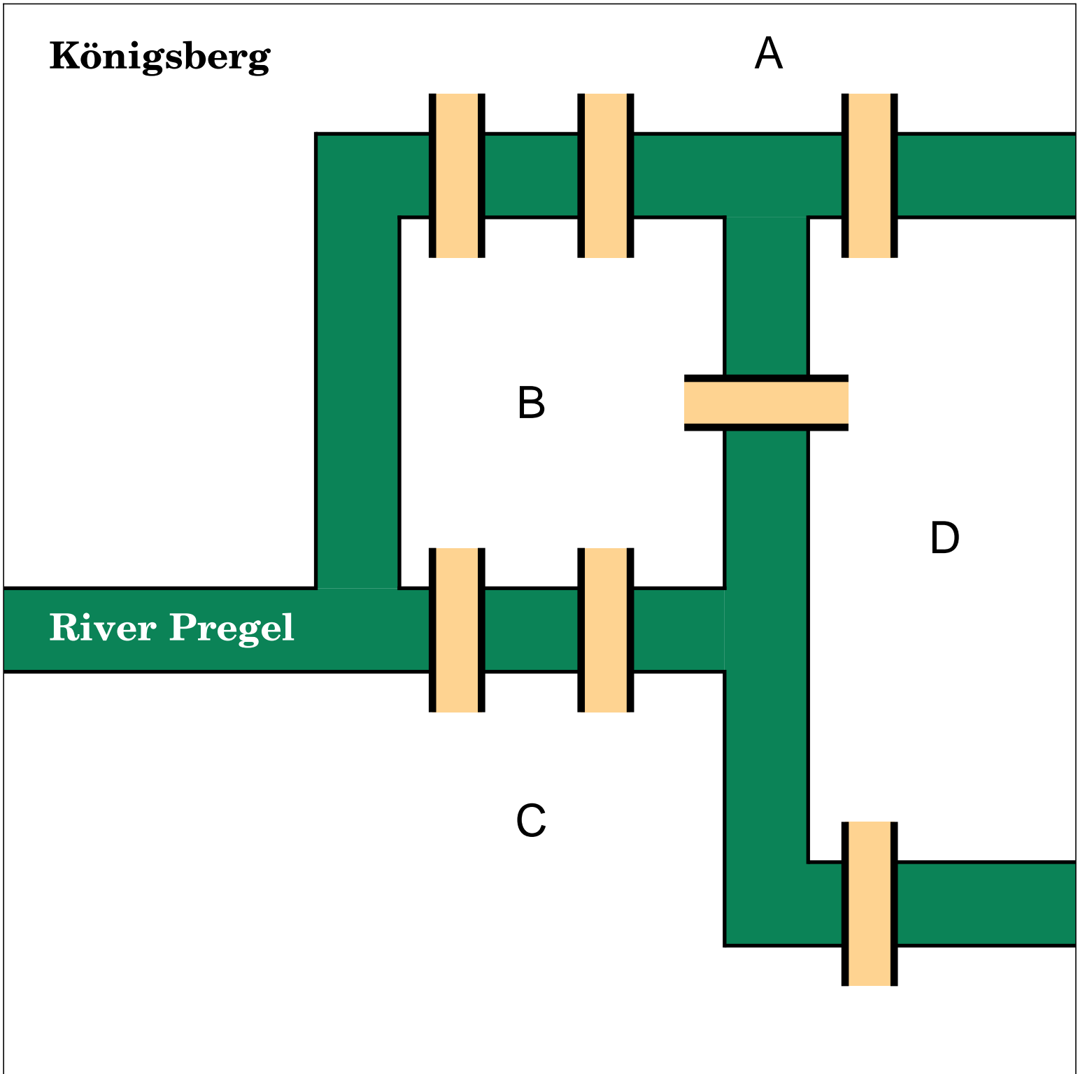
Figure 1 Bridges over the River Pregel, Königsberg, Prussia, 1736
